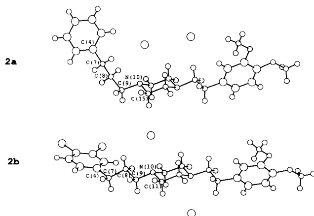
Figure 1. Structures of 2a and 2b found in their crystals.
