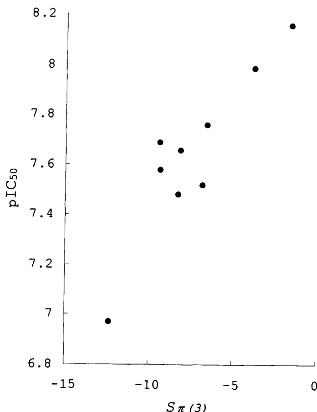
Figure 2. Correlation between S_{\pi(3)} and \sigma_1 -binding affinities ( pIC_{50} ). S_{\pi(3)} of 2i was calculated for 2i with a water molecule hydrogen-bonding to its 4-OH group.
