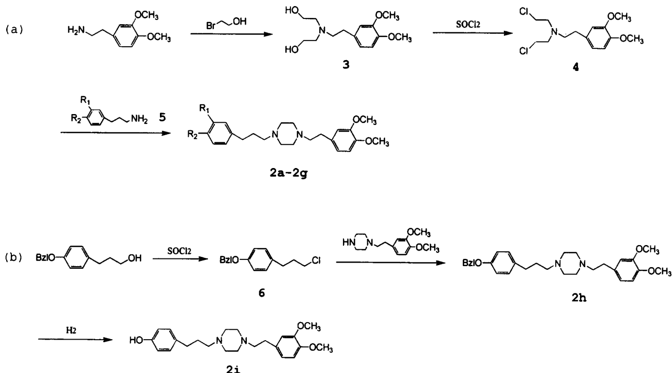
Scheme 1. Synthesis of 1-[2-(3,4-dimethoxyphenyl)ethyl]-4-(3-phenylpropyl)piperazines.
